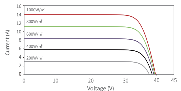
Current-Voltage Curves
