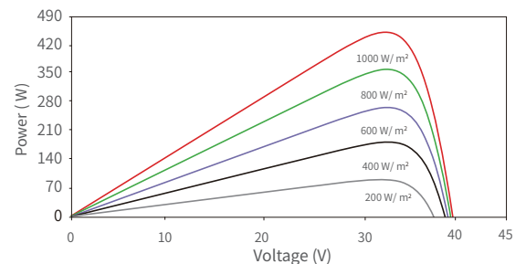
Power-Voltage Curves
